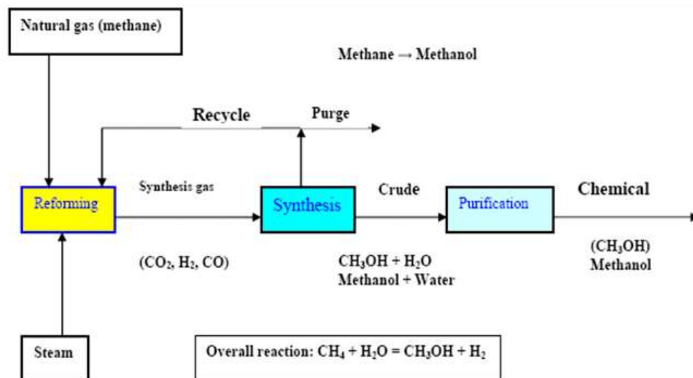
Figure 2: Schematic diagram shows methanol production (Omer, 2006).
