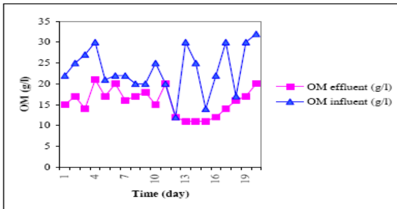
Figure 5. Organic matters before and after treatment in digester (Omer, 2006)
