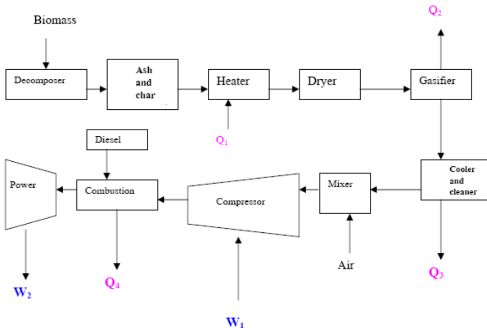
Figure 7. Advanced biomass power with diesel engine (Omer, 2006)
