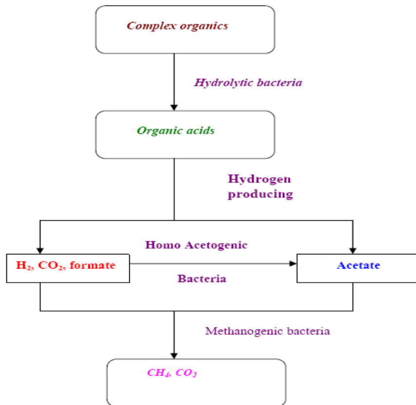
Figure 3; Biogas production process (Omer, 2003)
