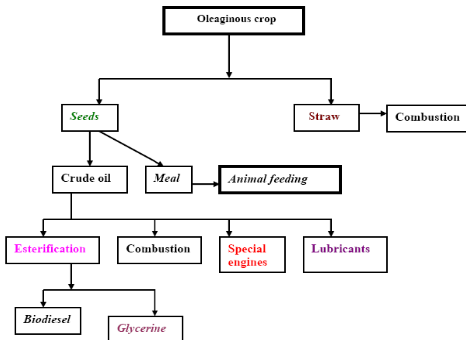
Figure 9. Flow chart of biodiesel production (Omer, 2006)
