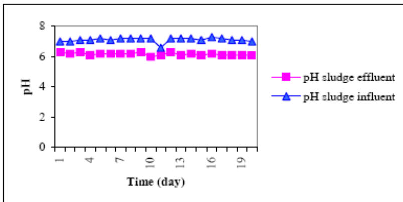
Figure 6: Potential of hydrogen (pH) sludge before and after treatment in the digester (Omer, 2006).
